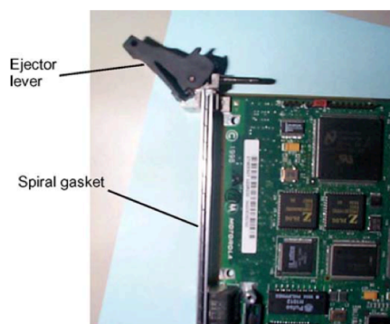
Figure 1 SDI35 CHASSIS
